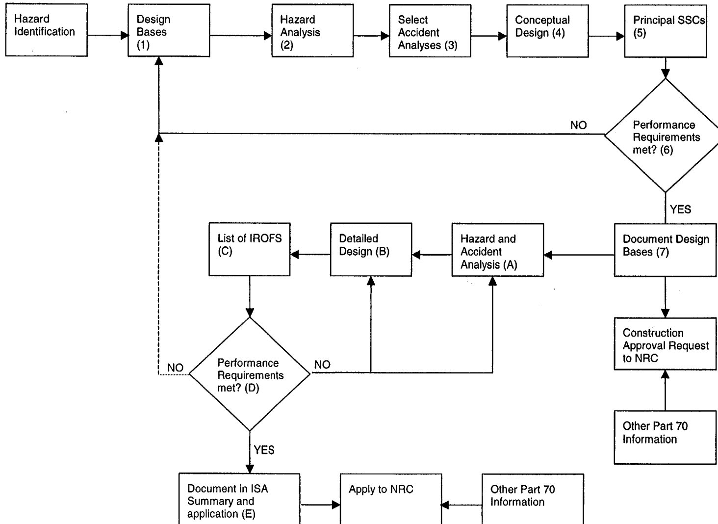
Figure 5-1: Relationship between the safety assessment of the design bases (Steps 1-7) and the ISA (Steps A-D)
