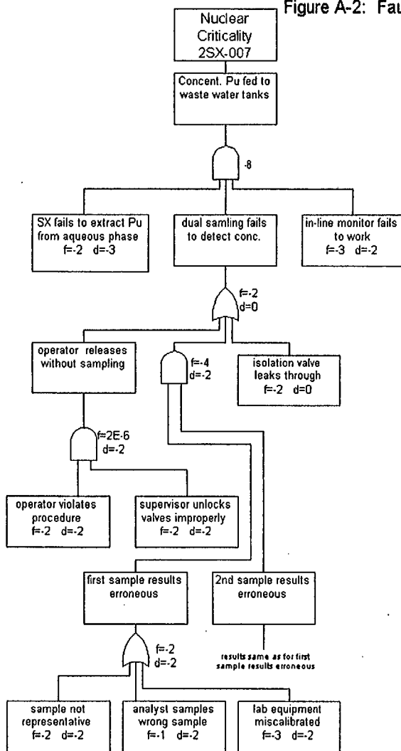
Figure A-2: Fault Tree for SX Operation (cont.)
