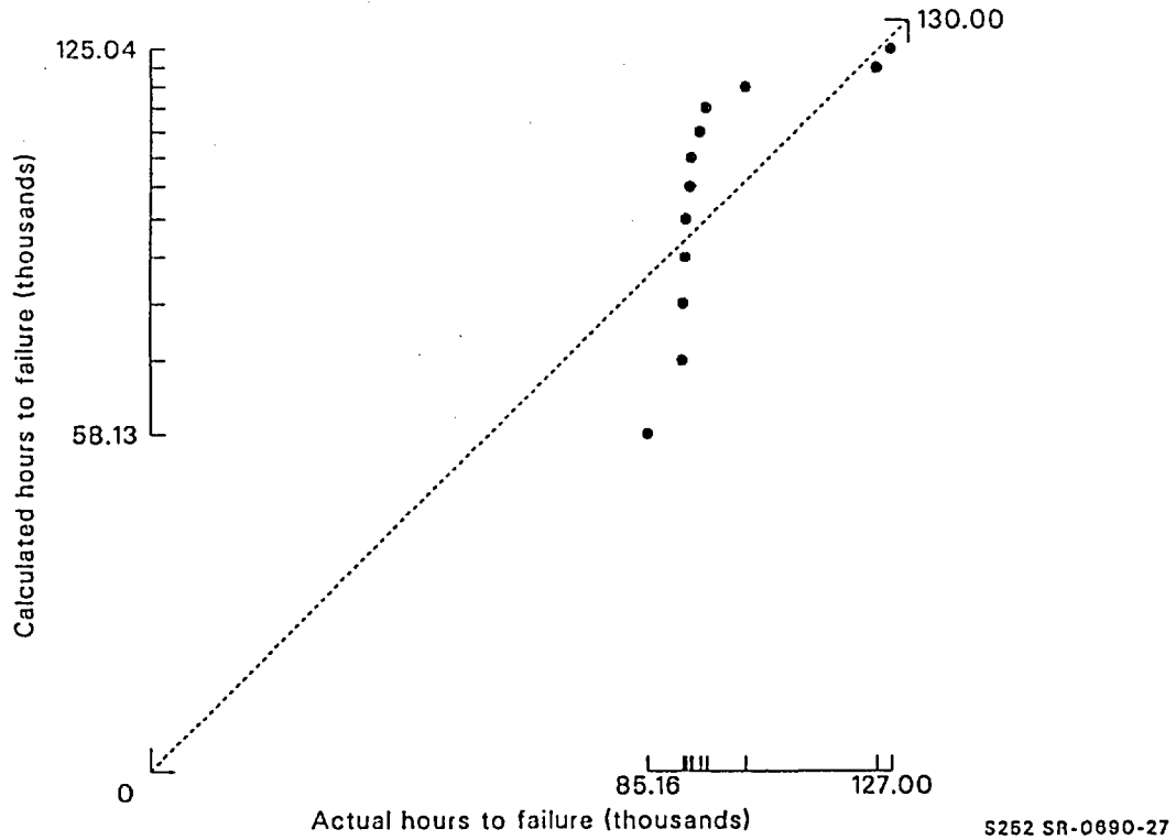
Figure 6-2. Q-Q plot for pump discharge check valves, broadly defined back leakage failures, exponential model, based on failures before the data were reinterpreted.
