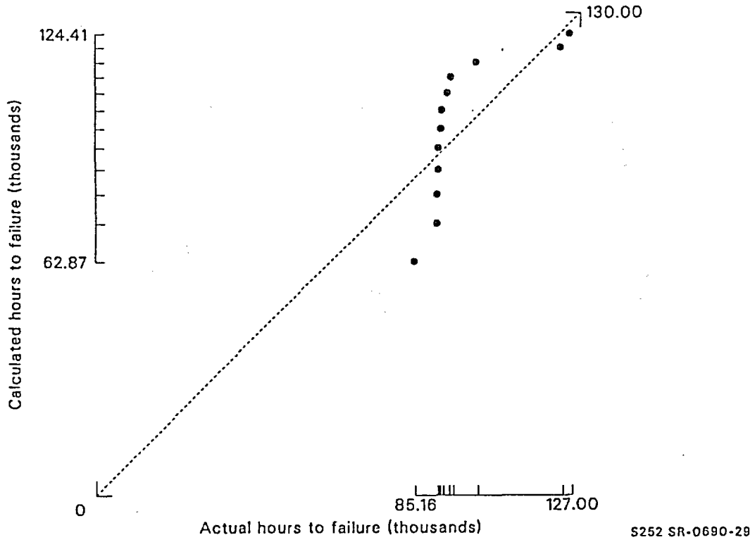
Figure 6-4. Q-Q plot for pump discharge check valves, broadly defined back leakage failures, linear model, based on failures before the data were reinterpreted.
