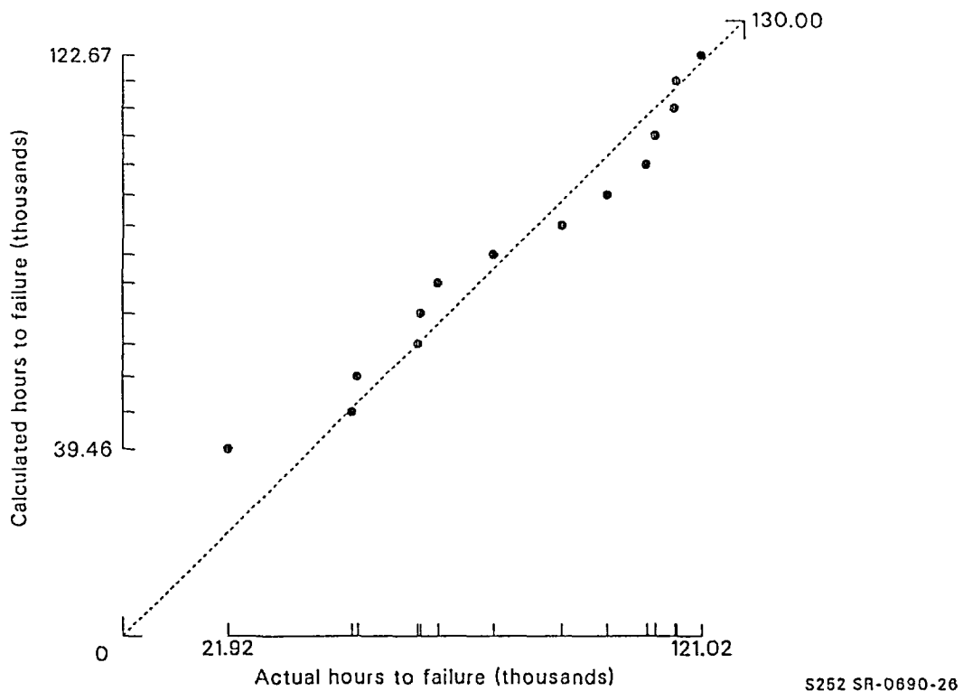
Figure 6-10. Q-Q plot for 3-in. MOVs (header isolation valves), narrowly defined plugging failures, linear model.
