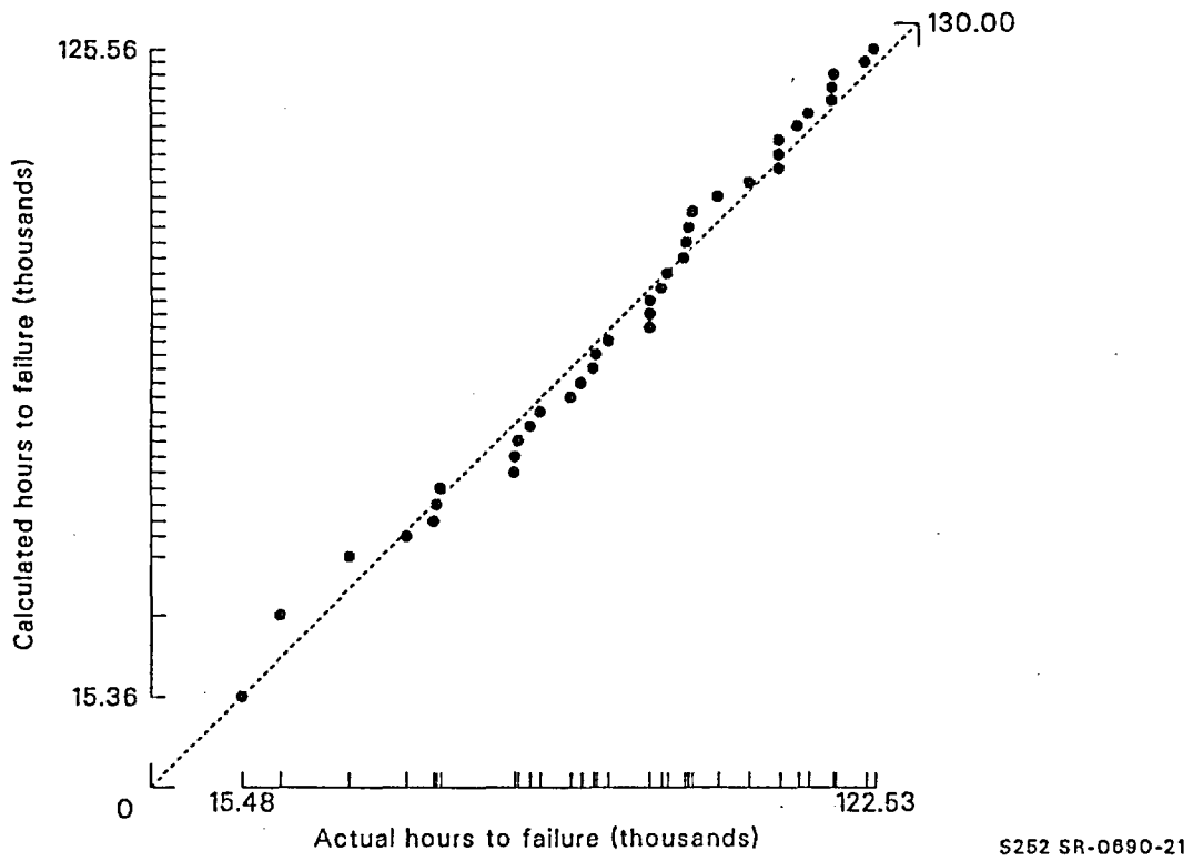
Figure 6-5. Q-Q plot for 3-in. MOVs (header isolation valves), broadly defined plugging failures, exponential model
