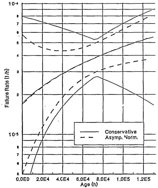
Figure 5-15. MLEs and 90% confidence bands for \lambda(t) , based on conservative calculations and on asymptotic normality for linear model.
