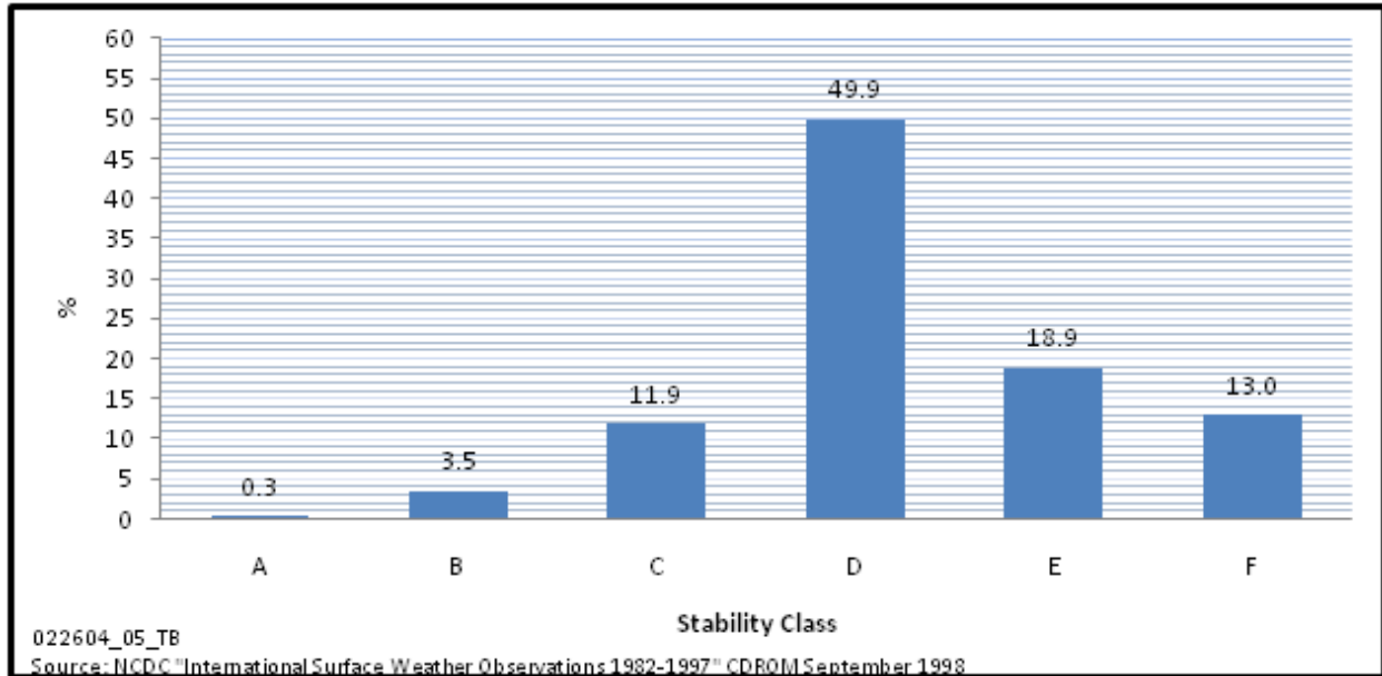
Figure 3- 59 Distribution of Stability Classes for Midland-Odessa, 1987-1991
