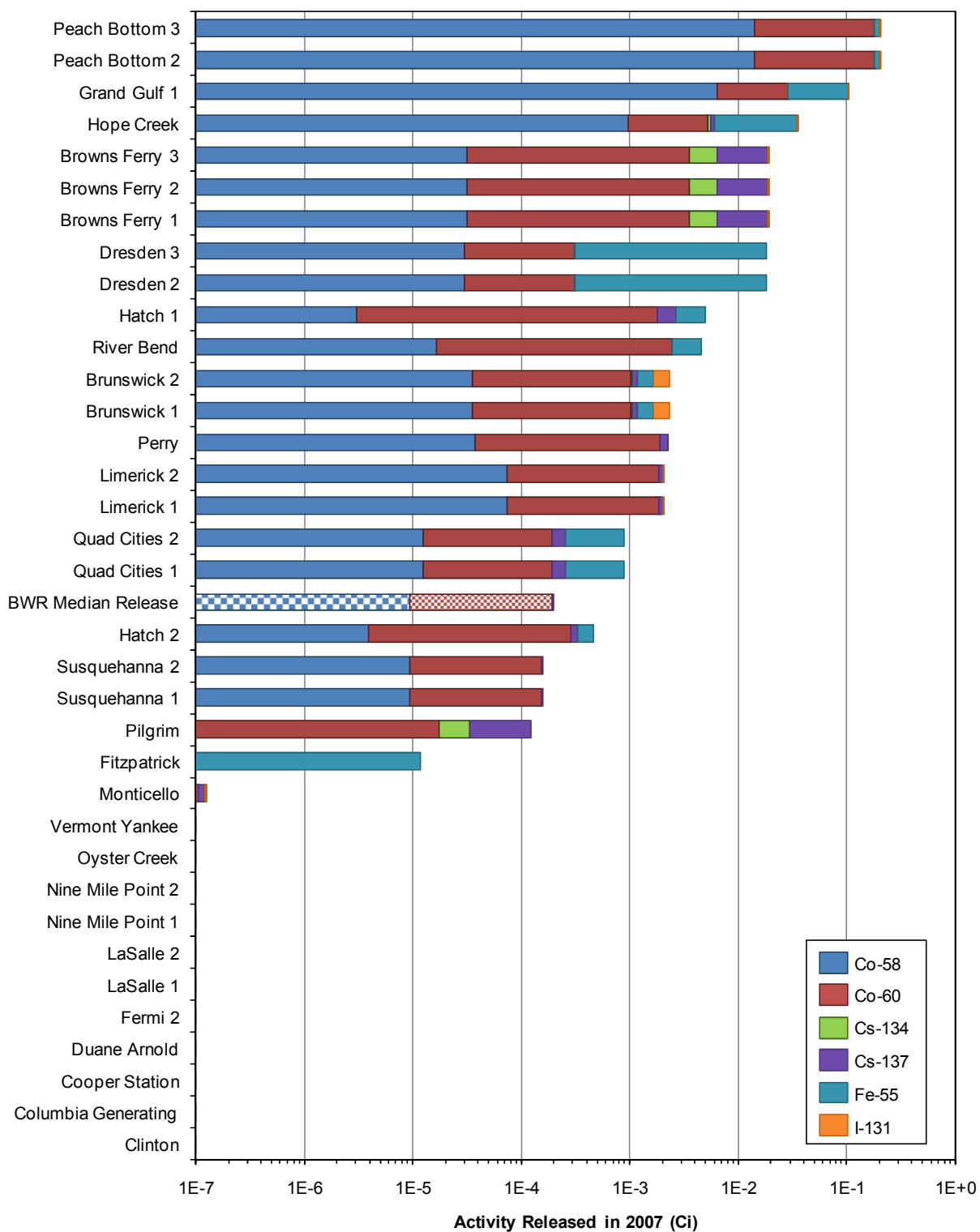
FIGURE 4.9 BWR Liquid Releases — Selected Fission and Activation Products
