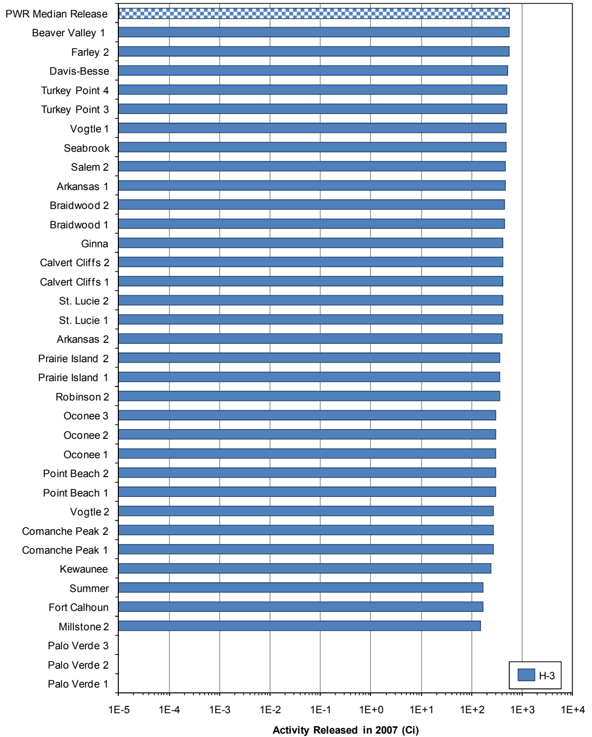
FIGURE 4.12 (continued) PWR Liquid Releases — Tritium
