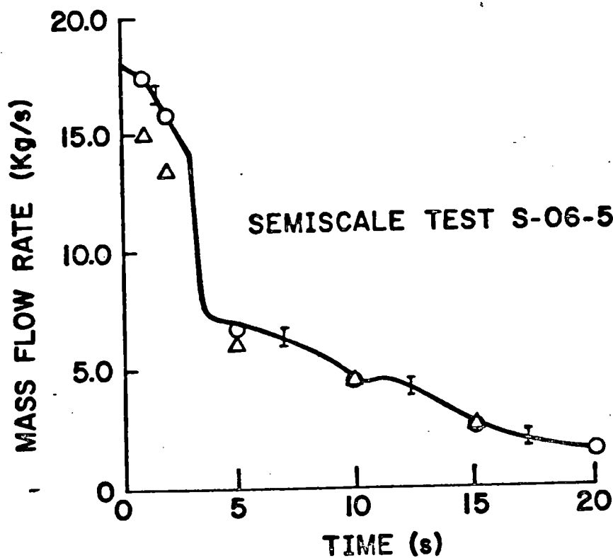
FIG. 3 Comparison of the measured mass flow rate (—) from Ref. 20, the computed mass flow rate with the nonequilibrium model (o), and the computed mass flow rate for equilibrium ( \Delta ).
