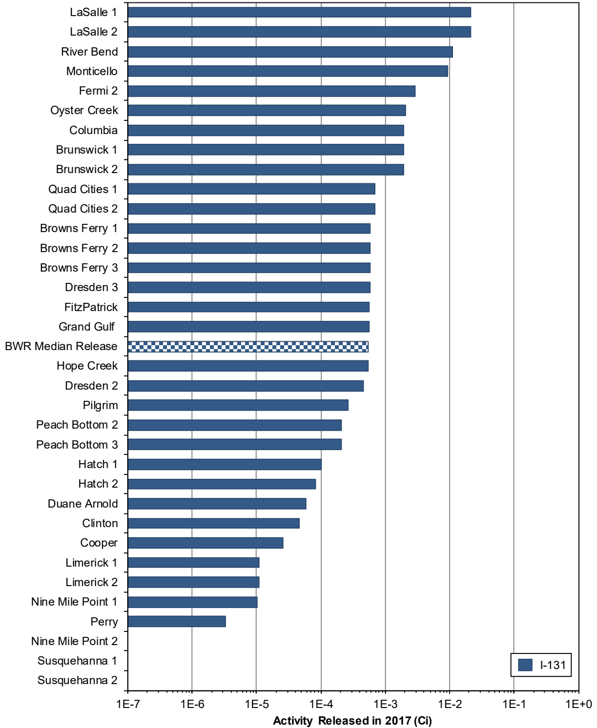
Figure 3.2 BWR Gaseous Releases — Iodine
