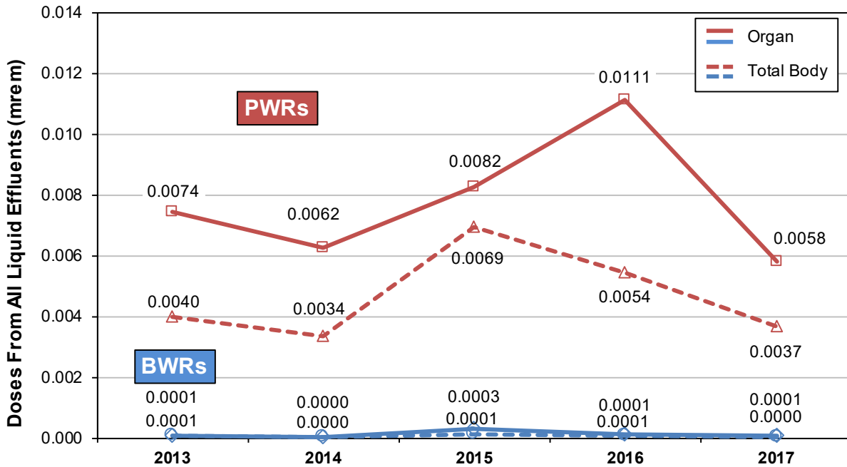
Figure 3.22 Median Maximum Annual Dose, Liquid Effluents 5-Year Trend, 2013-2017
