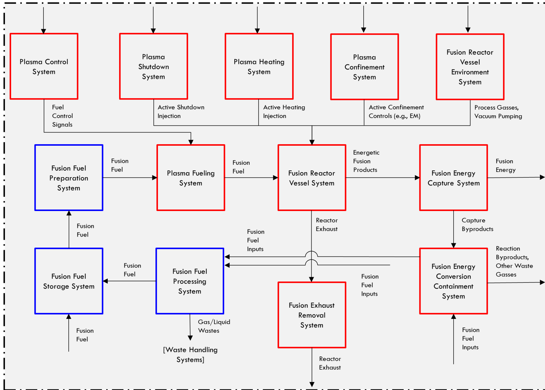
Portion of Level 3 System Engineering Model
