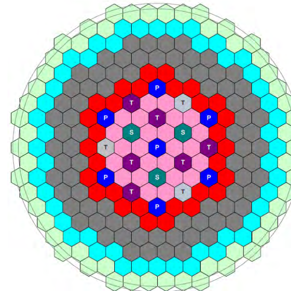
ABTR Core [2]
