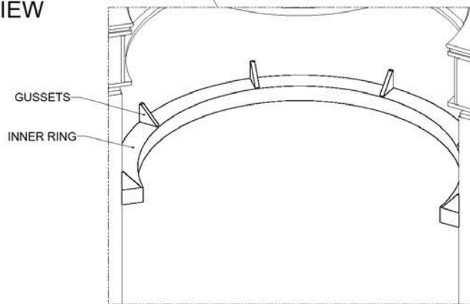
DETAIL VIEW
