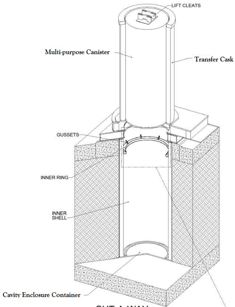
CUT-A-WAY ISOMETRIC VIEW
