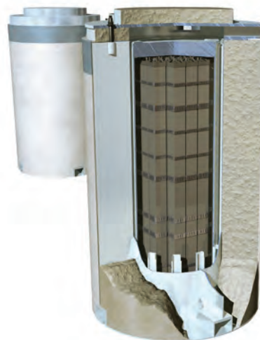
Cut-away View of Dry Spent Fuel Storage Container
