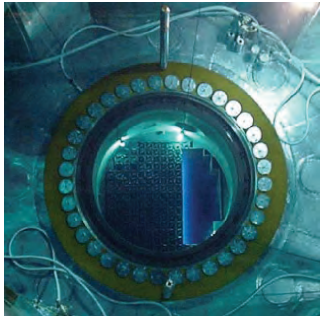
Looking Down at a Nuclear Reactor Core in the Reactor Vessel During Refueling Operations
